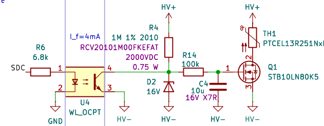
Discharge Circuit
