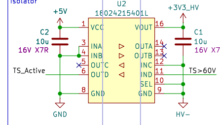
Isolator
