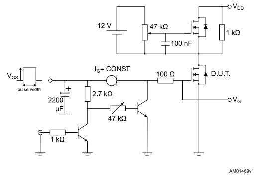
Figure 16: Test circuit for gate charge behavior
