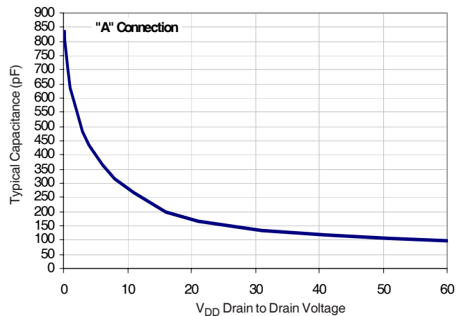
Figure 2. Typical Output Capacitance
