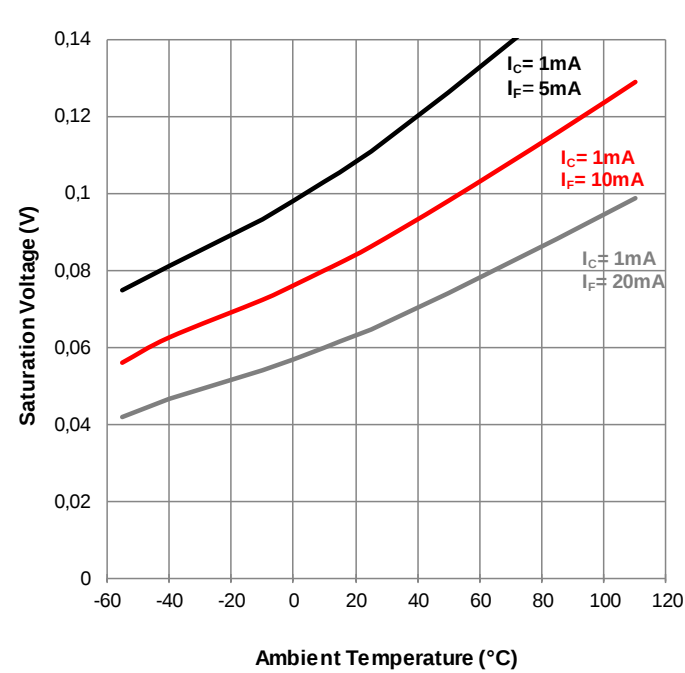
Collector-Emitter Saturation Voltage vs. Ambient Temperature:
