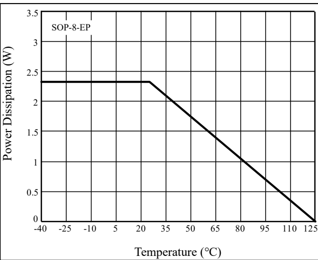
Figure 45 P_D vs. T_A
